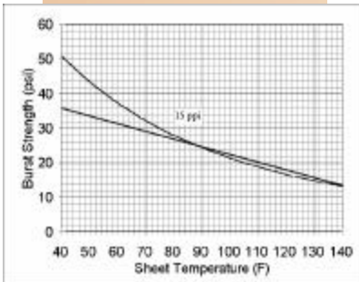
PVC Temperature vs Pressure Curve
